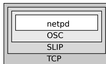
Figure 4: protocol stack
