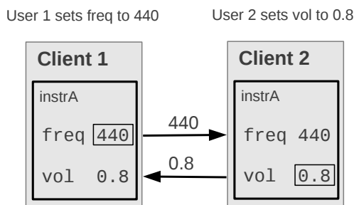
Figure 3: State synchronization
