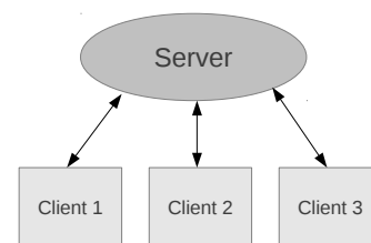
Figure 1: Client-server model
